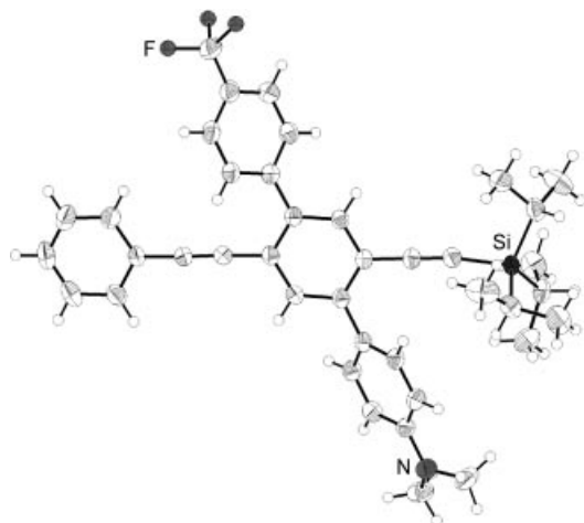
Figure 4. Solid state structure of 17 (ORTEP, thermal ellipsoids set at the 50% probability level).
