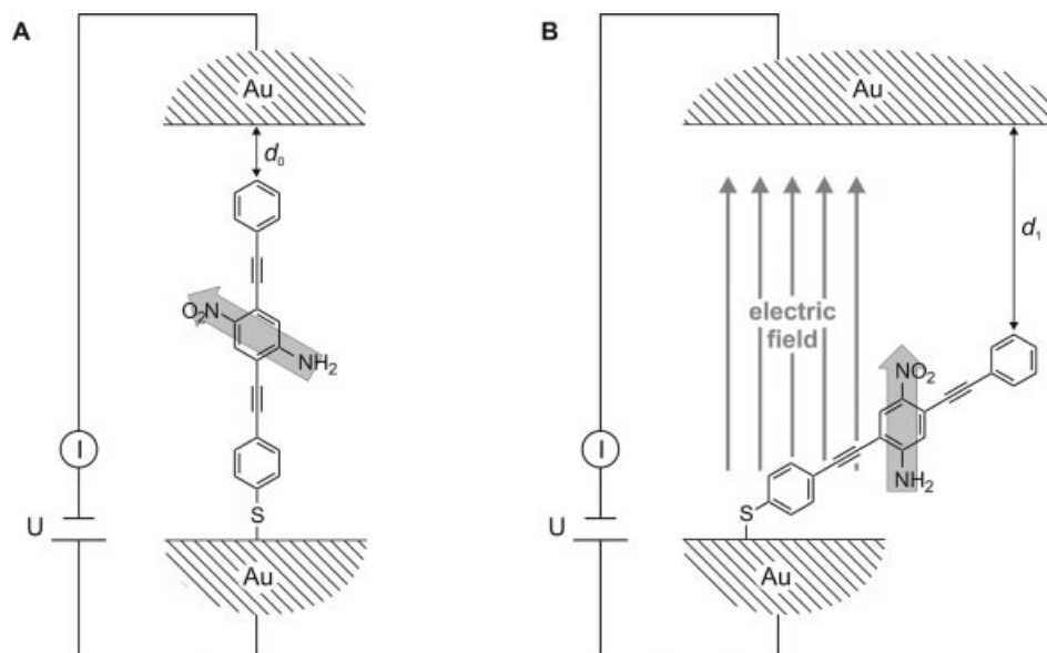
Figure 1. Sketch of a hypothetical switching mechanism of the reported NDR device. At low voltages the molecule stands more or less upright in the SAM with the distance d_0 for the tunnel current between the top electrode and the terminal \pi -system of the molecular rod (A). Upon applying an electric field, the para nitro aniline push-pull system of the central ring subunit aligns resulting in an increased distance d_1 between the top electrode and the end of the molecule (B).
