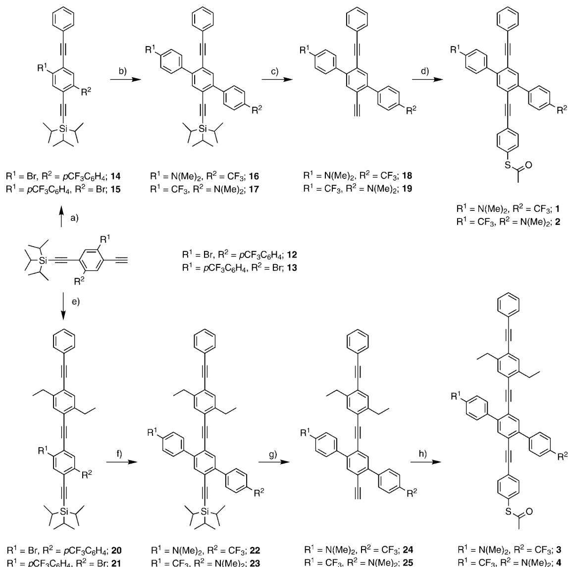
Scheme 3. Synthesis of target structures 1–4 . a) iodobenzene, \text{Pd}(\text{PPh}_3)_4 , (i\text{Pr})_2\text{NH} , \text{CuI} , THF, room temp., 16 h, 86% ( 14 ) and 86% ( 15 ); b) 4-(dimethylamino)phenylboronic acid, \text{Pd}(\text{PPh}_3)_4 , \text{K}_2\text{CO}_3 , \text{DME}/\text{H}_2\text{O} , 80^\circ\text{C} , 16 h, 84% ( 16 ) and 66% ( 17 ); c) TBAF, THF, room temp., 97% ( 18 ) and 94% ( 19 ); d) S -(4-iodophenyl) thioacetate, \text{Pd}(\text{PPh}_3)_4 , (i\text{Pr})_2\text{NEt} , \text{CuI} , THF, room temp., 16 h, 80% ( 1 ) and 83% ( 2 ); e) 1,4-diethyl-2-iodo-5-(phenylethynyl)benzene, \text{Pd}(\text{PPh}_3)_4 , (i\text{Pr})_2\text{NH} , \text{CuI} , THF, room temp., 16 h, 72% ( 20 ) and 90% ( 21 ); f) 4-(dimethylamino)phenylboronic acid, \text{Pd}(\text{PPh}_3)_4 , \text{K}_2\text{CO}_3 , \text{DME}/\text{H}_2\text{O} , 80^\circ\text{C} , 16 h, 86% ( 22 ) and 81% ( 23 ); g) TBAF, THF, room temp., 90% ( 24 ) and 96% ( 25 ); h) S -(4-iodophenyl) thioacetate, \text{Pd}(\text{PPh}_3)_4 , (i\text{Pr})_2\text{NEt} , \text{CuI} , THF, room temp., 16 h, 44% ( 3 ) and 62% ( 4 ).
