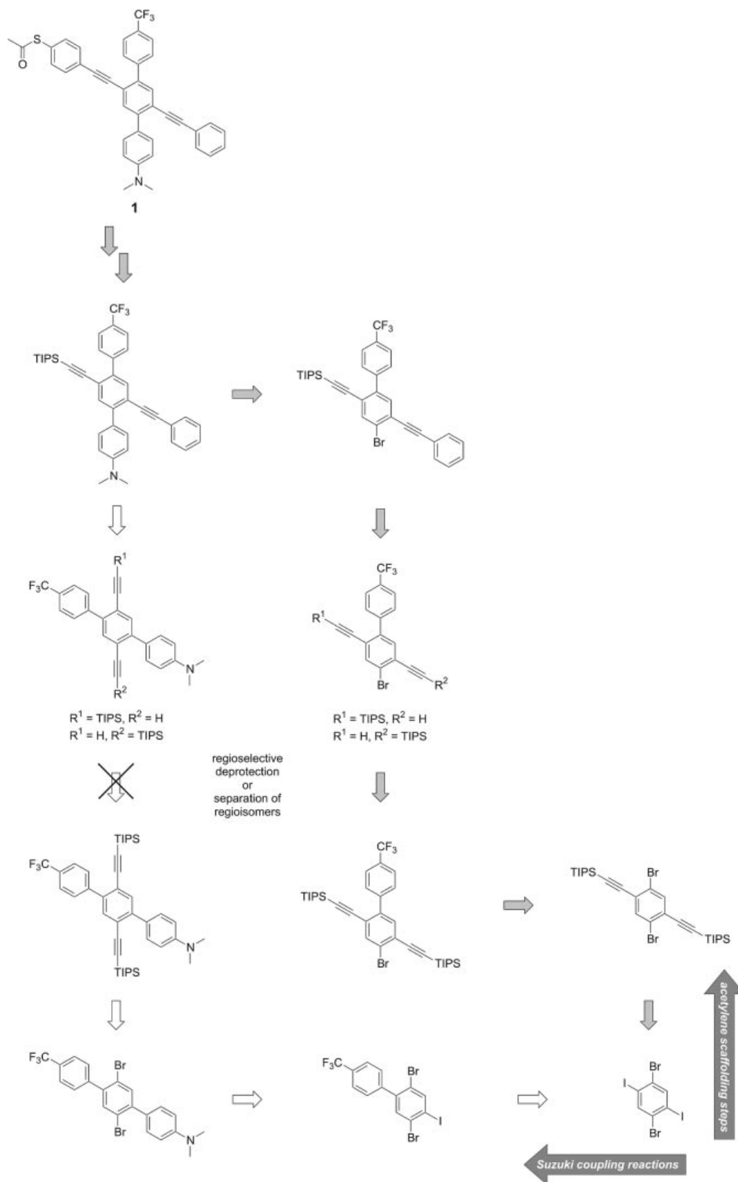
Figure 3. Retrosynthetic strategy to assemble the target structure 1 . Horizontal retrosynthetic arrows represent Suzuki coupling steps and vertical retrosynthetic arrows represent acetylene scaffolding steps like Sonogashira coupling reactions or acetylene deprotections. The white retrosynthetic arrows represent the pathway A , while the light grey retrosynthetic arrows display the synthetic path B which led to the target structure 1 .
