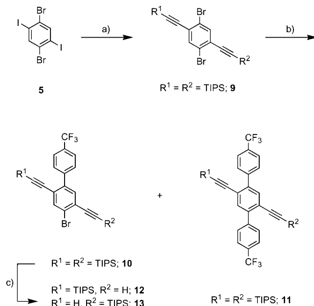
Scheme 2. Synthesis of both regioisomers 12 and 13 . a) TIPSA, Pd(PPh 3 ) 2 Cl 2 , ( i Pr) 2 NH, CuI, THF, room temp., 40 h, 77%; b) 4-(trifluoromethyl)phenylboronic acid, Pd(PPh 3 ) 4 , K 2 CO 3 , DME/H 2 O, 80 °C, 14 h, 46%; c) TBAF, THF/AcOH, room temp.
