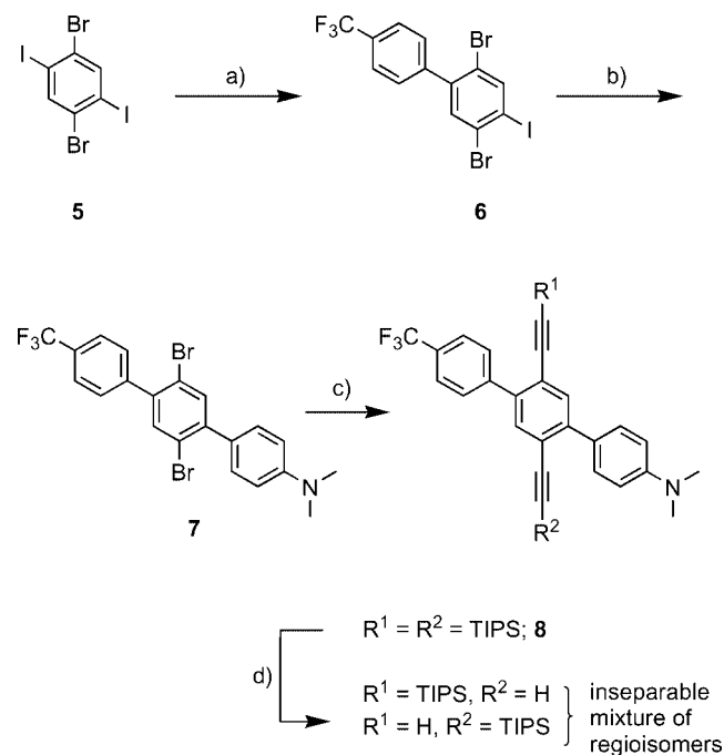
Scheme 1. Synthetic steps towards 1 following the retrosynthetic pathway A depicted in Figure 3: a) 4-(trifluoromethyl)phenylboronic acid, Pd(PPh 3 ) 4 , K 2 CO 3 , DME/H 2 O, 75 °C, 16 h, 48%; b) 4-(dimethylamino)phenylboronic acid, Pd(PPh 3 ) 4 , K 2 CO 3 , DME/H 2 O, 75 °C, 16 h, 15%; c) TIPSA, Pd(PPh 3 ) 2 Cl 2 , (iPr) 2 NH, CuI, THF, room temp., 16 h, 98%; d) TBAF, THF/AcOH, room temp.
